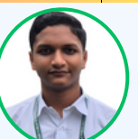
DIPTANSH SAIKIA 95.2%
